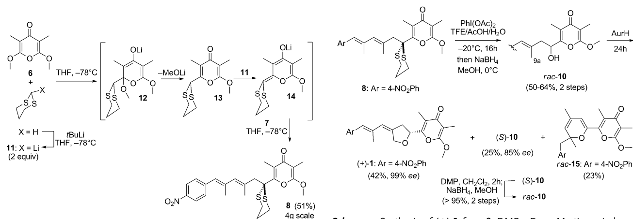
Scheme 3. One-pot preparation of 8 .
