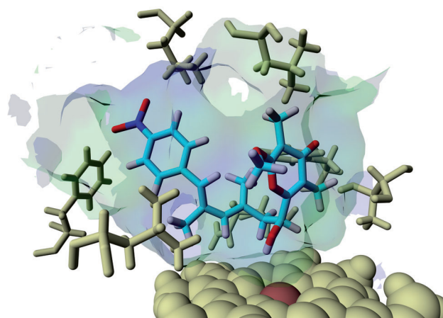
Figure 1. Model of substrate binding and AurH-mediated oxidation of ( S )- 10 to the corresponding ketone (EADock DSS).
